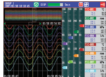
– Historical trend display – This display mode allows you to display historical data stored in memory.
