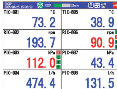
– Large-font digital display – The digital display mode shows measured data as numeric values, and displays channel number, tag name, engineering units, and alarm status.
