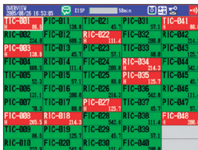
– Overview display – This screen lets you monitor the alarm status and numeric value for all channels.
