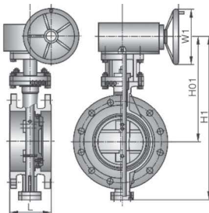
Worm Gear Driven Flanged Butterfly Valve
